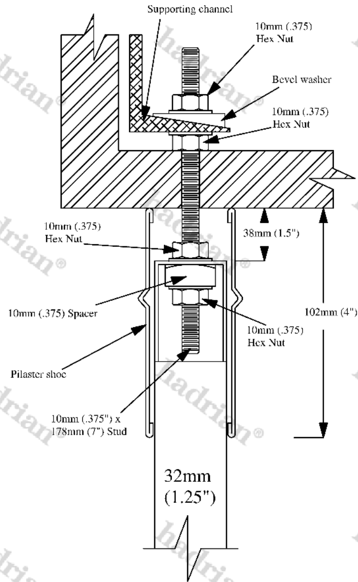
plan detail B-B
