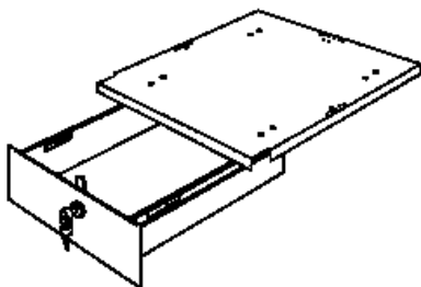
Drawer Assembly (Includes shelf, drawer with steel bearing slides, and fasteners. Drawer lock optional) #790058
